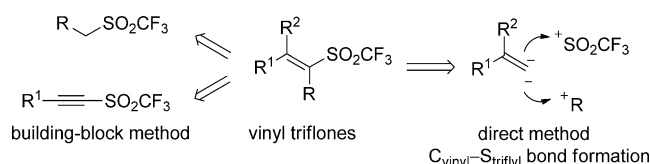
Figure 1. Strategies for substituted vinyl triflones: a building block method and a direct method ( \text{C}_{\text{vinyl}}-\text{S}_{\text{triflyl}} bond formation).
